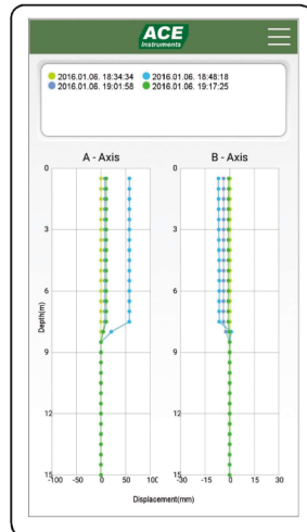
[스마트폰_Inclinometer Collector]
