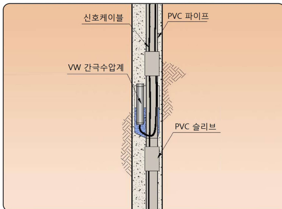
[단면도]
