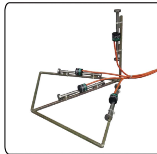
[4-방향용 Rosette Block]
