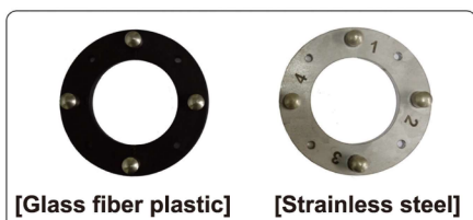
[Tilt Plate]
